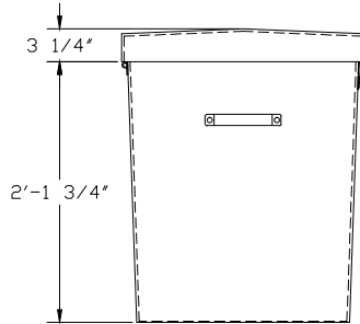
LEFT ELEVATION
