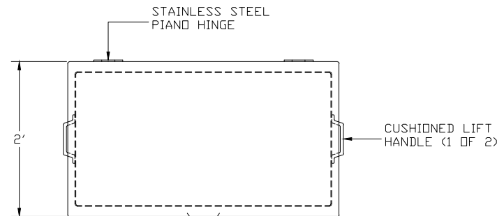
PLAN VIEW
